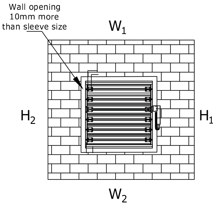
Clearance of MFSD (Front View)
