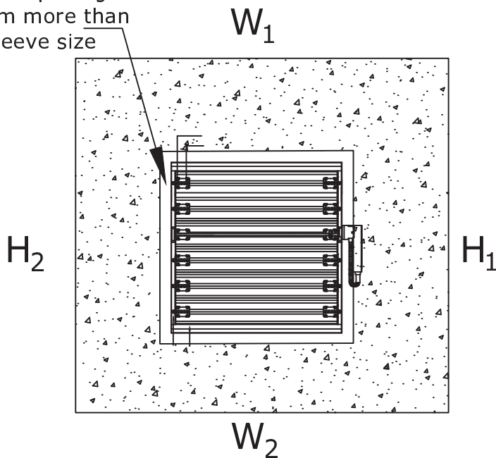
Clearance of MFSD (Top View)
